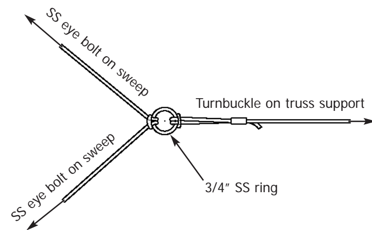
Figure 4 SS ring Assembly
