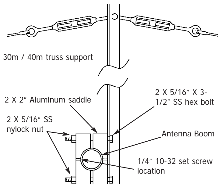
Figure 3 Coupler Assembly
